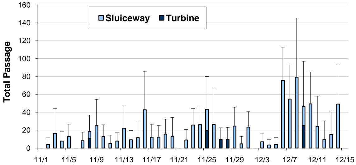
Figure 3.3. Number of Overwintering Summer Steelhead Targets Passing Daily at Each Route of the Powerhouse and Sluiceway from November 1 – December 15, 2009 (error bars depict the 95% CI)
