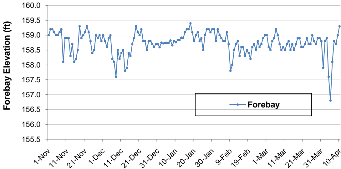
Figure 3.2. Forebay Elevation (ft above MSL) at TDA During the Entire Study Period (November 1, 2009 – April 10, 2010). Forebay data were obtained from DART ( http://www.cbr.washington.edu/dart/dart.html ), accessed on July 10, 2010 and from TDA Operations.
