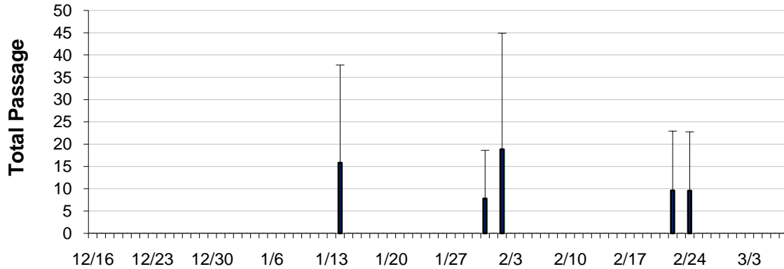
Figure 3.7. Number of Overwintering Summer Steelhead Targets Passing Daily at Each Route of the Powerhouse from December 16, 2009 to March, 7 2010 (95% CI)
