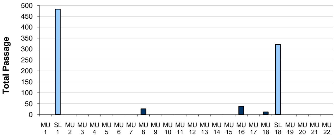
Figure 3.4. Horizontal Distribution of Overwintering Summer Steelhead Targets Passage at Each Route of the Powerhouse and Sluiceway from November 1 – December 15, 2009 (MU = main unit, SL = sluice)
