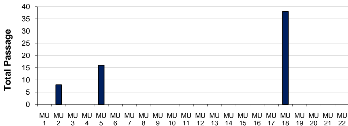
Figure 3.8. Horizontal Distribution of Overwintering Summer Steelhead Targets Passage at Each Route of the Powerhouse from December 16, 2009 to March 7, 2010 (MU = main unit)
